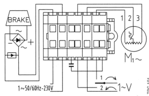
Monofase con freno 1-phase with brake
