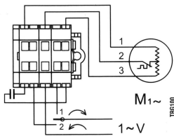
Monofase 1-phase
