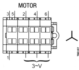
Trifase a stella Star 3-phase
